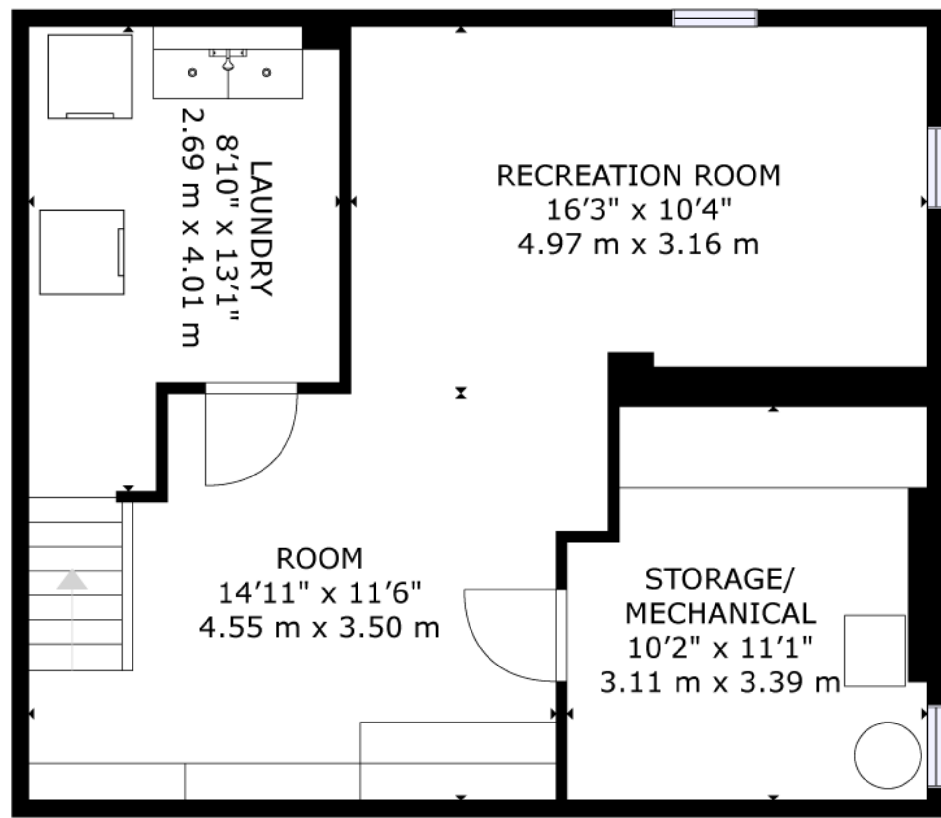
BASEMENT 1
